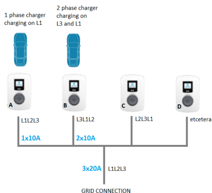
Figure 6.6: 2 phase EV connected to an SCN, reduced charging current
