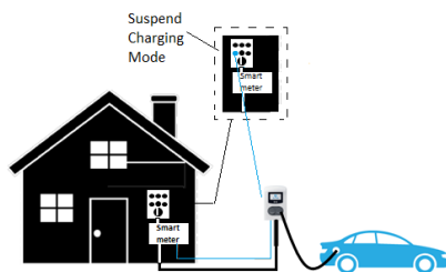
Figure 8.2: Scenario Suspend Charging Mode with potential free contact (energy meter)
