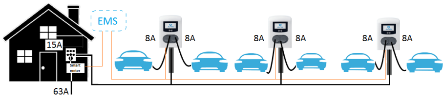
Figure 5.9: Scenario ALB in combination with smart energy meter, EMS and multiple charging stations
