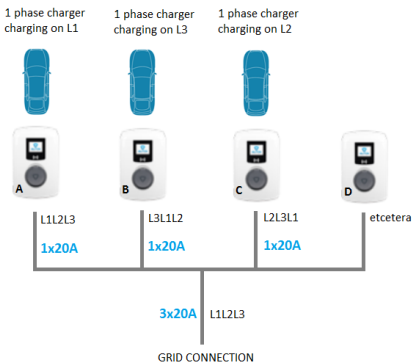
Figure 6.4: Single phase EVs connected to SCN, optimal charging current
