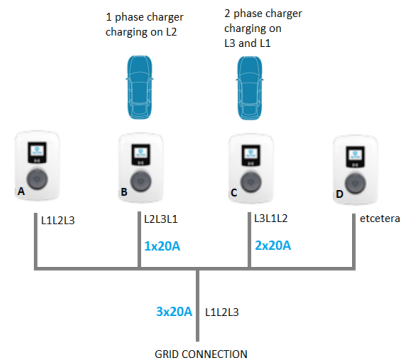
Figure 6.5: 2 phase EV connected to an SCN, optimal charging current
