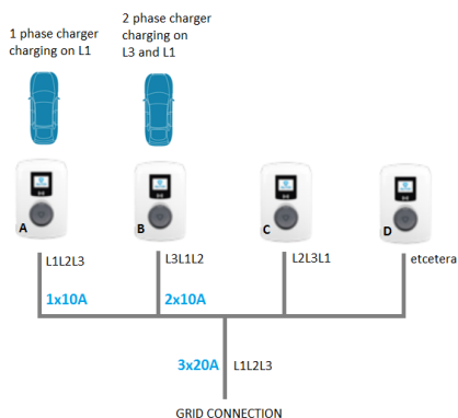
Figure 6.7: 3 phase EV connected to an SCN, reduced charging current
