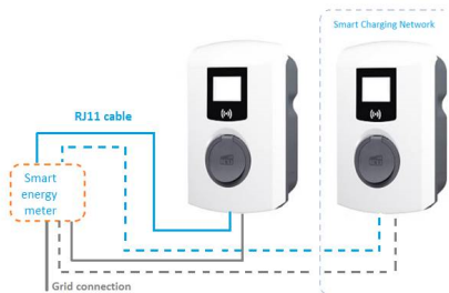
Figure 5.2: Active Load Balancing with energy meter (P1 part)
