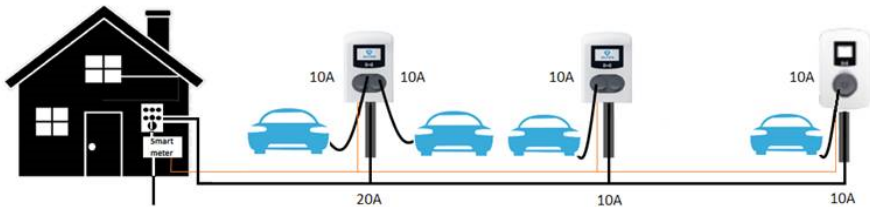
Figure 6.2: SCN with double socket charging stations
