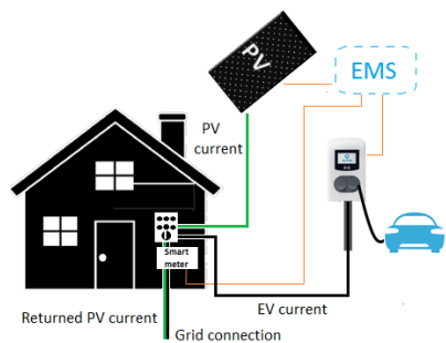
Figure 5.1.2: Scenario ALB in combination with smart energy meter, EMS and integrated PV
