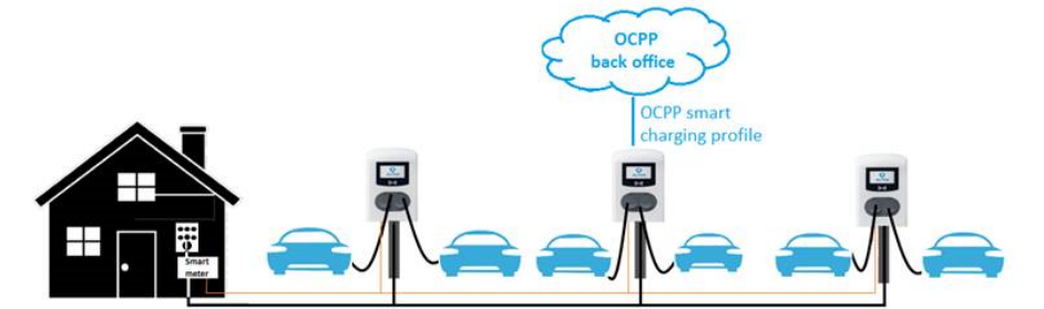
Figure 9.3: Scenario OCPP Smart Charging in an SCN
