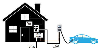
Figure 5.6: scenario ALB in combination with smart energy meter
