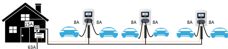
Figure 5.7: Scenario ALB in combination with smart energy meter and multiple charging stations
