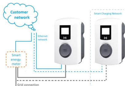
Figure 5.3: Active Load Balancing with energy meter (Modbus TCP/IP)
