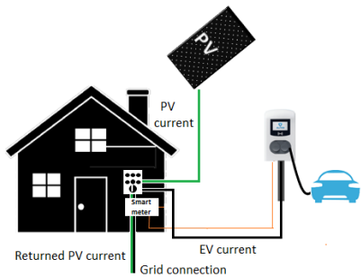
Figure 5.10: Scenario ALB in combination with Smart energy meter and integrated PV
