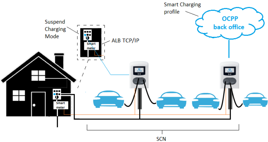
Figure 9.1: Combination of ALB, SCN, Suspend Charging Mode and OCPP Smart Charging profile
