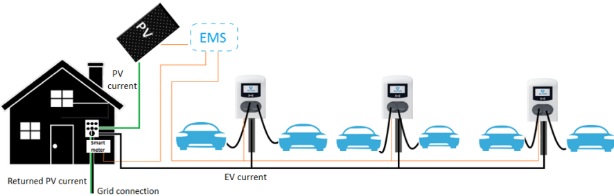
Figure 5.1.3: Scenario ALB in combination with smart energy meter, EMS, SCN and integrated PV
