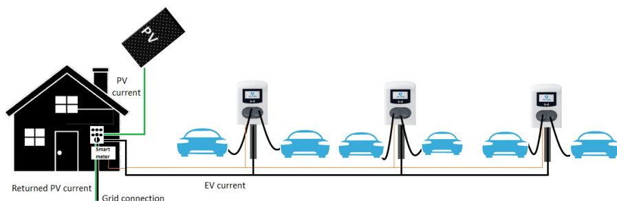
Figure 5.11: Scenario ALB in combination with smart energy meter, SCN and integrated PV
