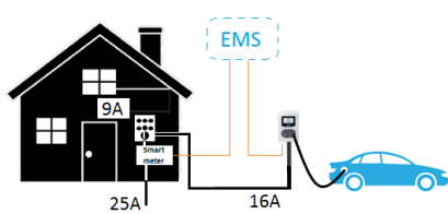
Figure 5.8: Scenario ALB in combination with Smart energy meter and EMS
