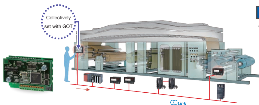
Connection to CC-Link network with LE7-CCL network option
