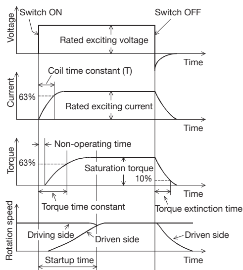
Fig. 3 Operating characteristics of powder clutch
