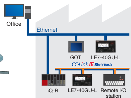
Ethernet saves man-hours and enables long-distance transmission
