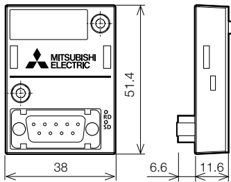
FX5-232-BD
