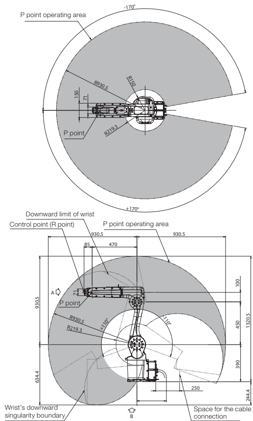
View B: Detailed installation dimensions
