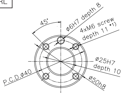
View C: Detail of mechanical interface
