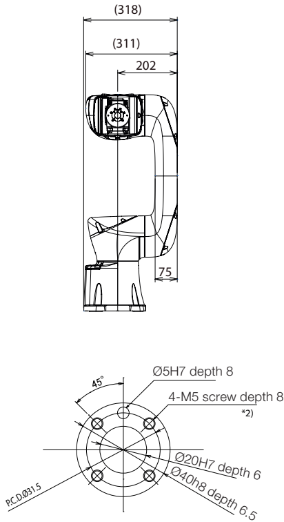
View A: Detail of mechanical interface *2) The depth in which the screw is tightened is 7.5 to 8 mm.
