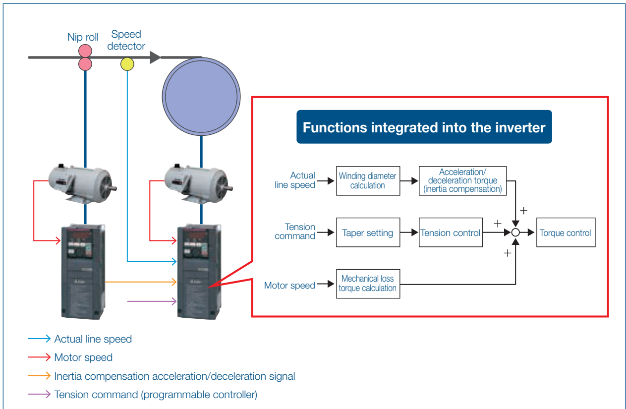
Example of tension sensorless torque control
