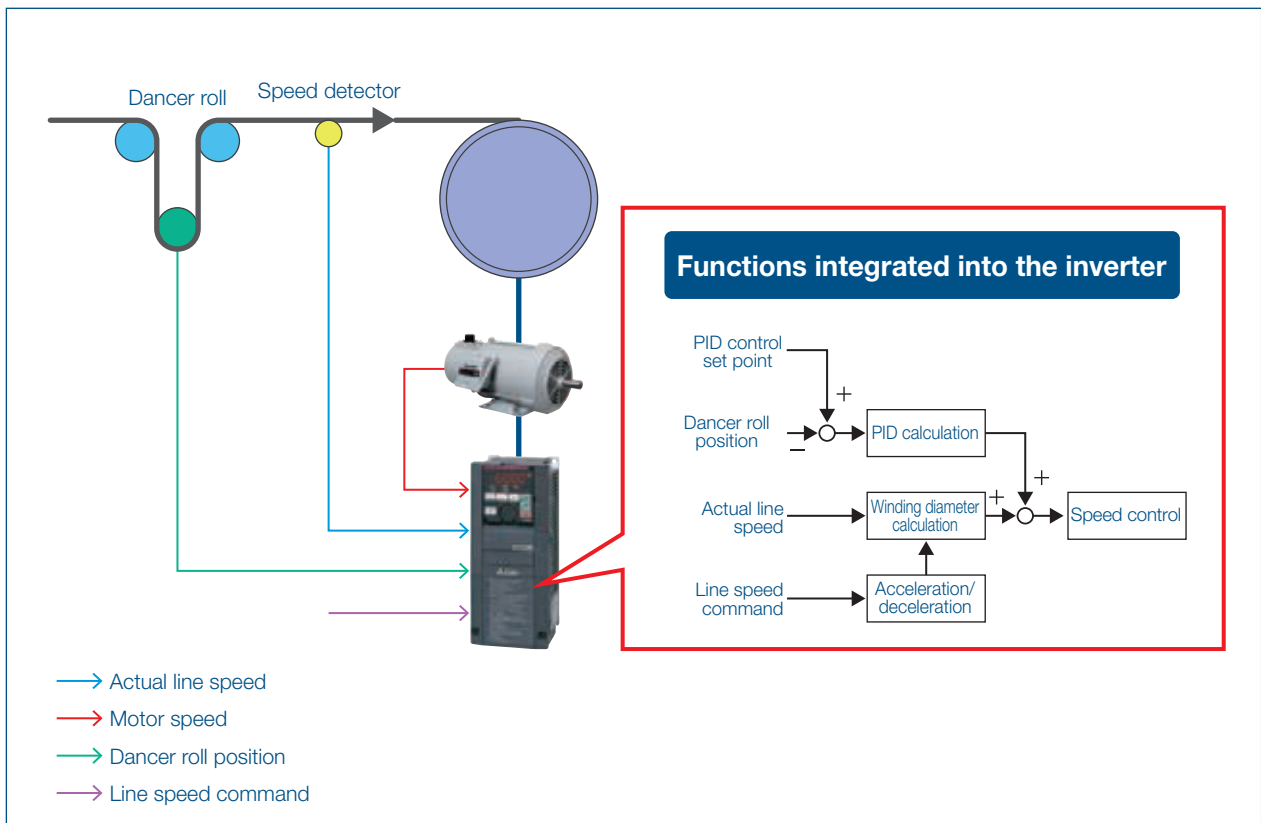
Example of dancer feedback speed control
