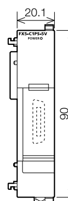
FX5-C1PS-5V
