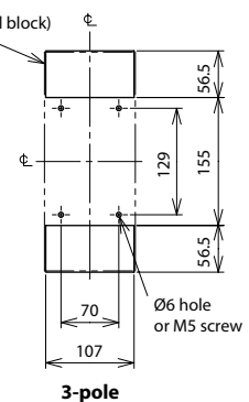
Drilling plan
