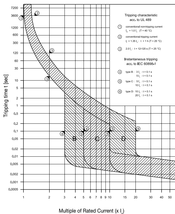
Characteristics B, C and D - UL 489
