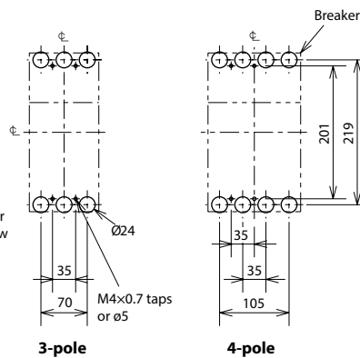
Drilling plan
