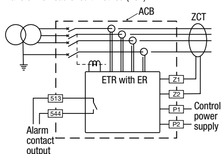
Transformer load circuit method (ZCT)
