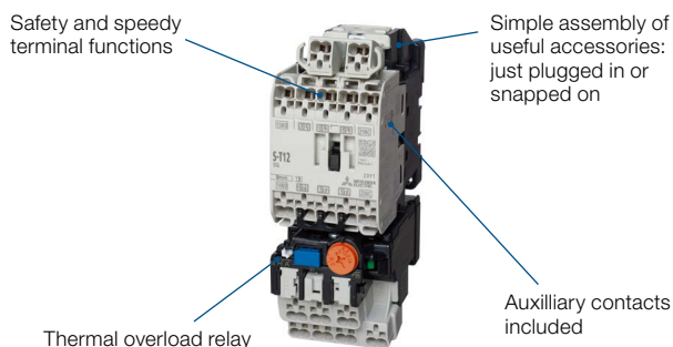
Magnetic contactor with mounted thermal overload relay of the MS series
