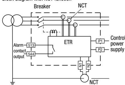
Block diagram with NCT function
