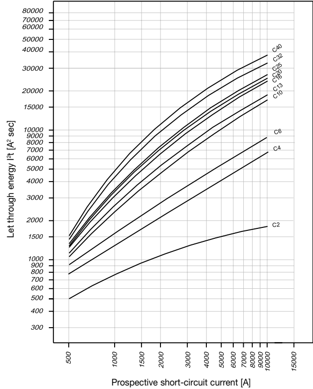
Let-through Energy RCBO, Characteristic C, 1+Npolig
