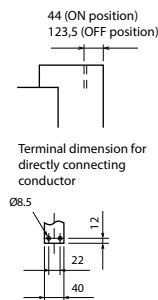
Conductor drilling for direct connection
