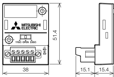
FX5-485-BD
