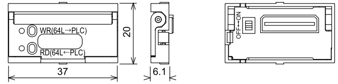
FX3U-FLROM-16/64/64L
