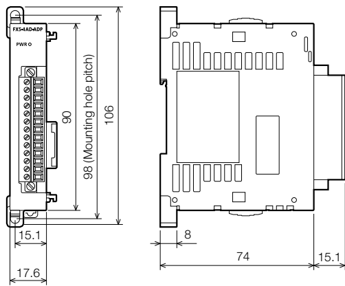
FX5-4AD-ADP/FX5-4DA-ADP FX5-4AD-PT-ADP/FX5-4AD-TC-ADP
