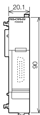
FX5-C1PS-5V
