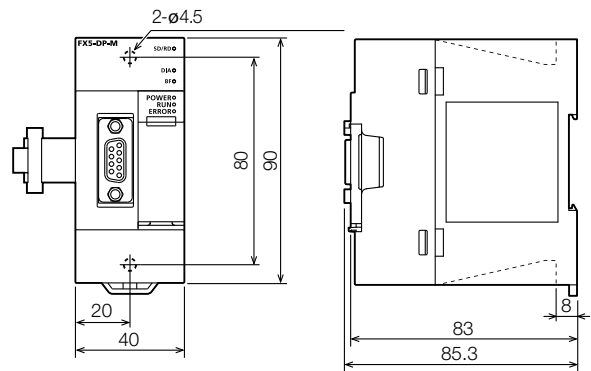
FX5-DP-M
