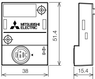
FX5-422-BD-GOT
