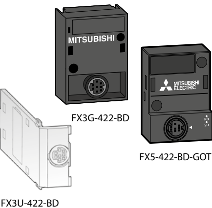
FX3U-422-BD
