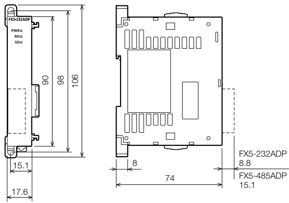
FX5-232ADP/FX5-485ADP
