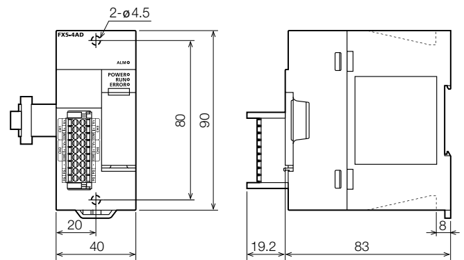
FX54AD, FX5-4DA
