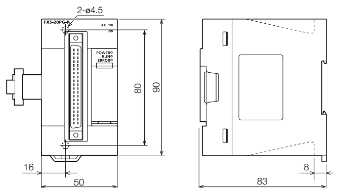
FX5-20PG-P
