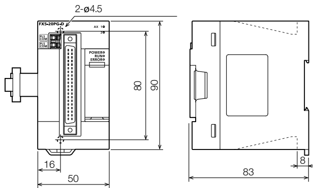
FX5-20PG-D
