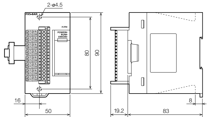
FX5-8AD
