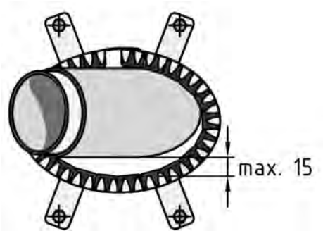
Fig. 42: Maximum allowable gap between pipe and fire protection collar.
