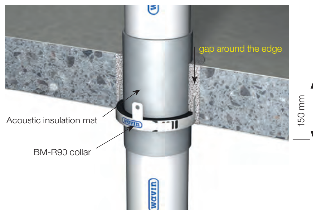
Fig. 40: Straight installation with / without sleeve / socket.
