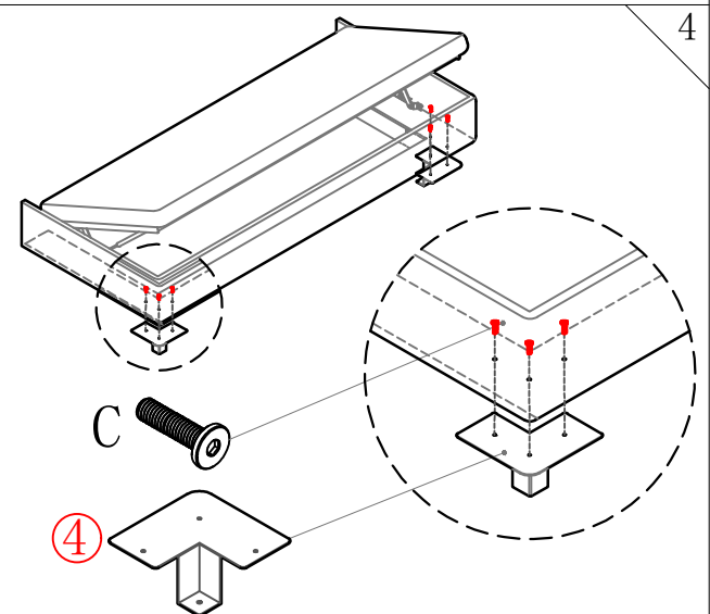
CORNER METAL LEGS INSTALLATION
