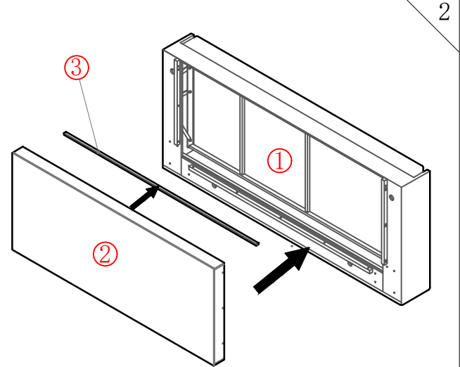
UPPER - LOWER BOX INSTALLATION
