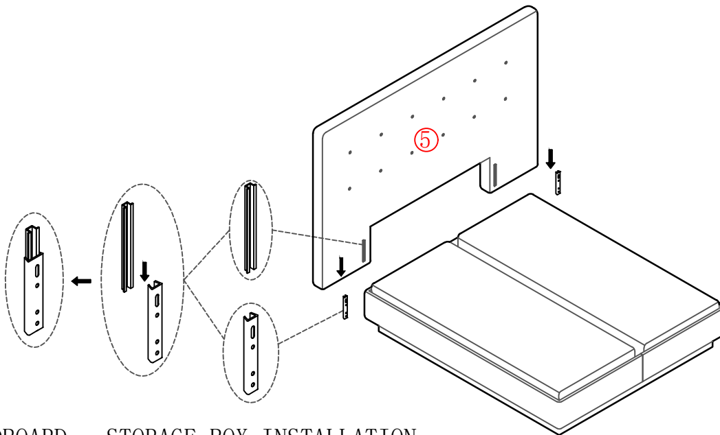
HEADBOARD - STORAGE BOX INSTALLATION
