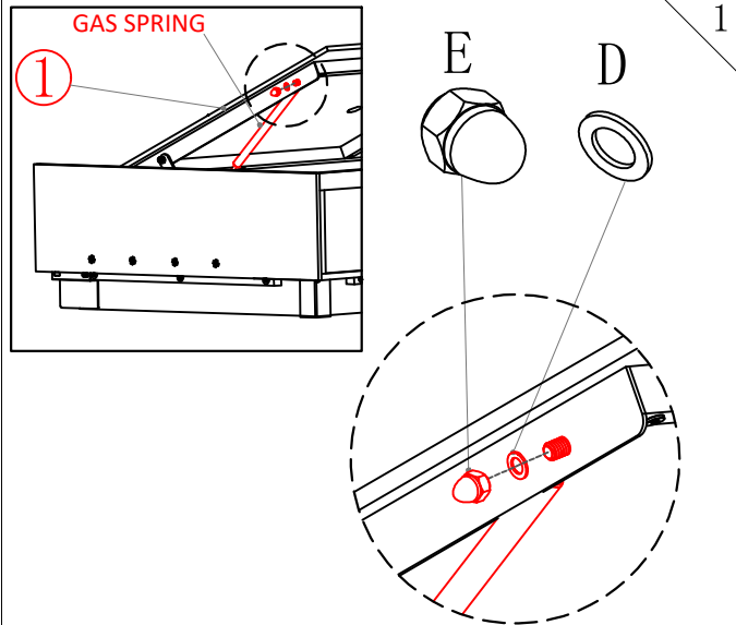
GAS SPRING INSTALLATION
