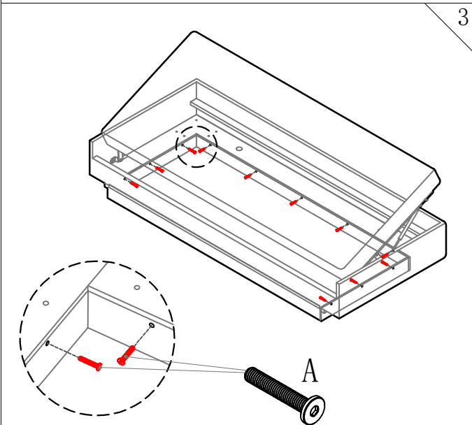
GAS SPRING INSTALLATION
