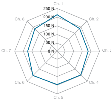
Evenly distributed radial load for uniform sealing even at small diameters.
