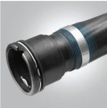
Oetiker's Multi Crimp Rings are a robust and proven connecting technology for Battery Tempering, Onboard Electronics Cooling and eMotor Cooling.
