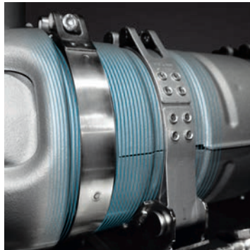
Oetiker's high performance products excel in maintaining mechanical integrity and sealing under vibration, stress and temperature in Exhaust Aftertreatment Systems and Engine Exhaust connections.
