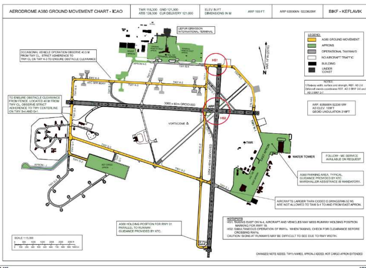
This chart is also published in AD 2.24 BIKF Ground Movement Chart -ICAO in AIP BIKF.
