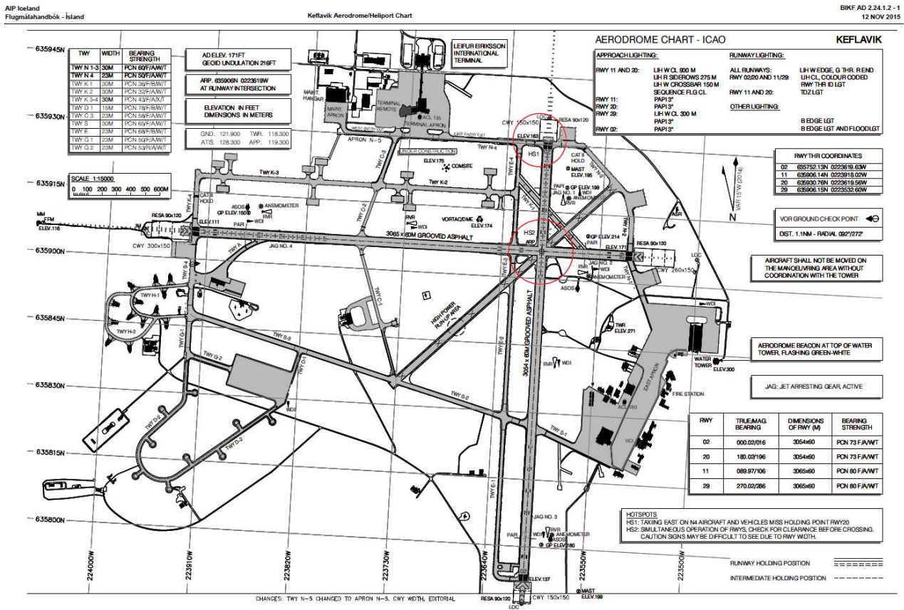
Aerodrome chart. This chart is also published in AIP BIKF AD 2.24
